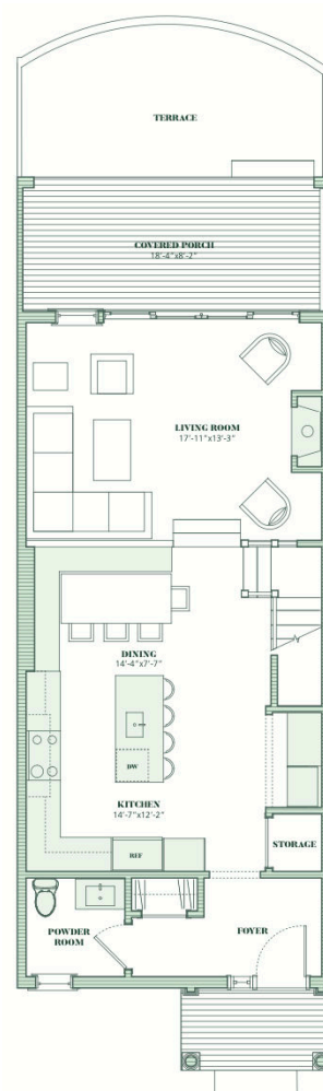
First Floor
